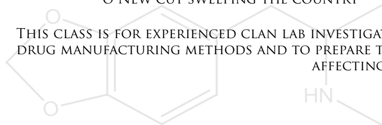
3,4-Methylenedioxyamphetamine
